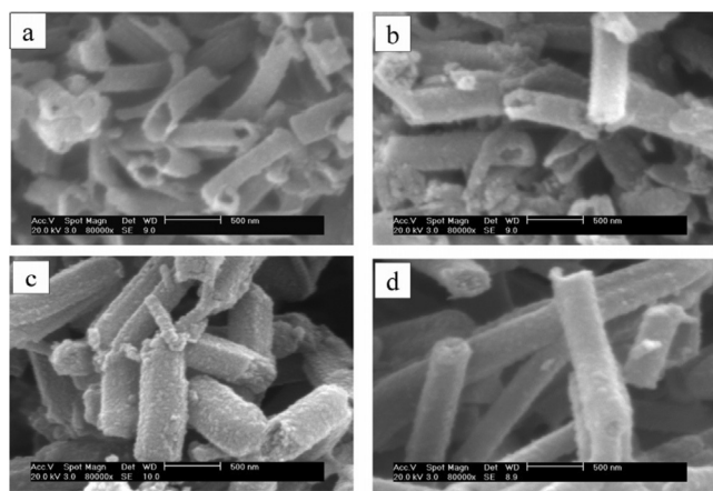
Figure 5. SEM images of graphitic mesoporous carbon materials using various mesoporous silica SBA-15 rods as templates at different aging temperatures: a) 40°C, b) 70°C, c) 100°C, and d) 130°C. [28c] Scale bars: 500 nm. Copyright 2005 American Chemical Society.
