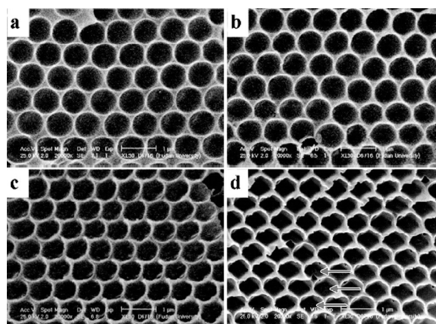
Figure 3. SEM images of the hierarchically ordered meso/macroporous silica samples using a) 0.1, b) 0.3, c) 0.5, and d) 0.8 g of 2 M HCl solution. [24] Scale bars: 1 \mu\text{m} . Copyright 2011 American Chemical Society.
