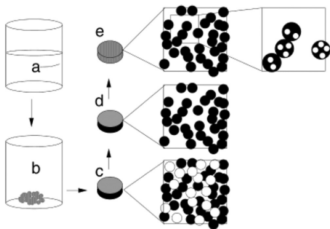
Figure 8. Generation of macroporous materials starting with the combustion synthetic preparation of an intimate mixture of two metal oxides. Starting from \text{Ni}^{\text{II}} and \text{Zn}^{\text{II}} nitrates in solution with urea as the fuel “a”, combustion synthesis yields an intimate mixture of the oxides “b”, which is sintered to form the monolith “c”. The ZnO in monolith is leached by alkali to yield a macroporous oxide “d”. Reduction of “d” should yield macroporous Ni metal “e”, but closer examination reveals that, in addition, ZnO is removed from “d” on reduction, giving rise to another level of porosity. [42d] Copyright 2002 American Chemical Society.
