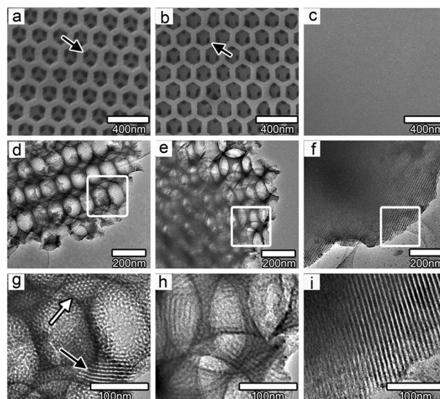
Figure 17. SEM/TEM micrographs of macro-mesoporous \text{TiO}_2 films without (a,d,g) and with (b,e,h) graphene, and purely mesoporous \text{TiO}_2 film (c,f,i). The black arrows in (a,b) indicate the interconnected channels between macropores in the films, whereas the white and black arrows in (g) suggest the mesopores in the macroporous walls. [77] Copyright 2010 American Chemical Society.
