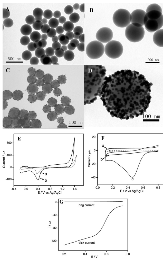
Figure 19. A,B) TEM image of TiO 2 precursor spheres at different magnifications. C,D) TEM images of TiO 2 (precursor sphere)/Au hybrid spheres at different magnifications. [103a] E) CVs of CPB (line a)- and RHAHS (line b)-modified GC electrode (5 mm) in a N 2 -sparged 0.5 M H 2 SO 4 solution; F) CVs of O 2 reduction at RHAHS-modified gold electrode (lines b and c) and bare gold electrode (line a) in air-saturated (lines a and c) and N 2 -saturated (line b) 0.5 M H 2 SO 4 solution; G) Current-potential curves for the reduction of O 2 at a rotating platinum ring-GC (5 mm) disk electrode with RHAHS adsorbed on the disk electrode in the presence of air (experimental conditions: 1 V constant ring potential, 500 rpm rotation rate, 50 mV s -1 scan rate, 0.5 M H 2 SO 4 solution). [103a] Copyright 2009 American Chemical Society.
