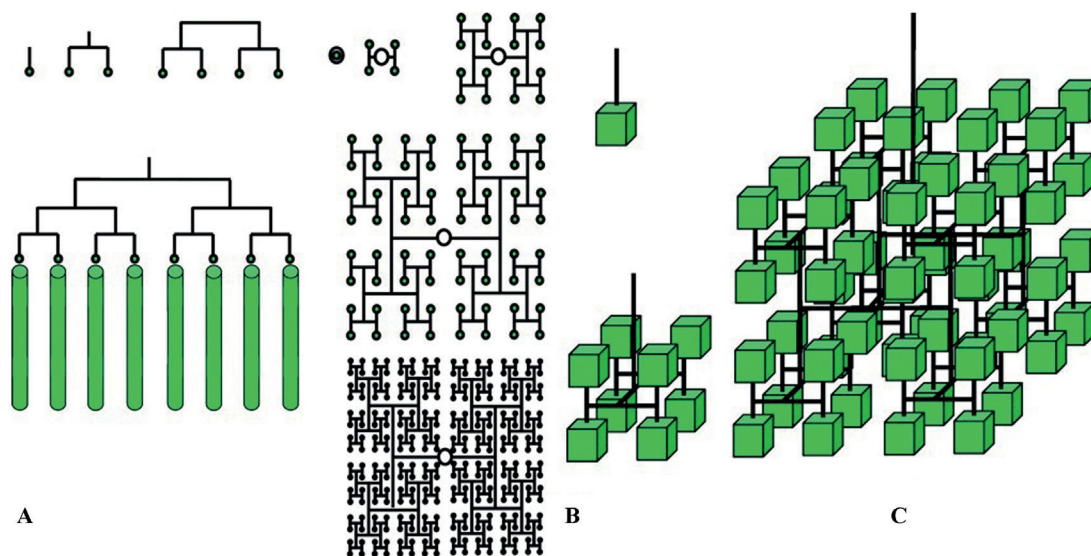
Figure 25. A) A set of 1D distributors feeding progressively larger 1D arrays (vectors). B,C) Extension of the scalable, fractal distributor concept to 2D and 3D, respectively.
