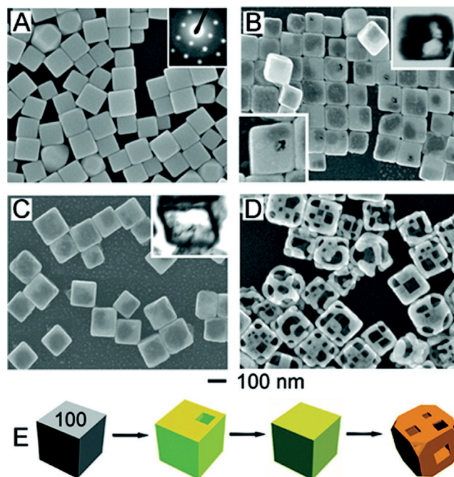
Figure 7. A) SEM of Ag nanocubes. B) SEM of product after addition of 0.30 mL of 1 mM \text{HAuCl}_4 solution to a 5 mL 0.8 mM Ag nanocube suspension; a pinhole (lower inset) is observed on the exposed face of approximately 1 in 6 nanocubes and TEM (upper inset) of a microtomed sample reveals early hollowing out. C) SEM of product after addition of 0.50 mL of \text{HAuCl}_4 solution. TEM (inset) of a microtomed sample reveals the hollow interior of the nanobox. D) SEM of product after addition of 2.25 mL of \text{HAuCl}_4 solution. Porous nanocages are produced. e) illustration summarizing morphological changes. [33b] Copyright 2008 American Chemical Society.
