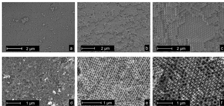
Figure 13. SEM images of the colloidal crystal templates (top) and associated \text{LiFePO}_4 templated samples calcined at 500^\circ\text{C} (bottom) formed using PMMA beads of diameter 100 nm (a,d), 140 nm (b,e), and 270 nm (c,f), respectively. [60b] Copyright 2009 American Chemical Society.
