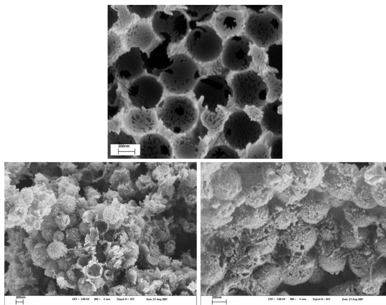
Figure 1. SEM images of the macroporous carbon nitride template with 500 nm pores (CN-500) (top) and the obtained TiN-500 (bottom). [13a] Scale bars: 200 nm. Copyright 2008 American Chemical Society.
