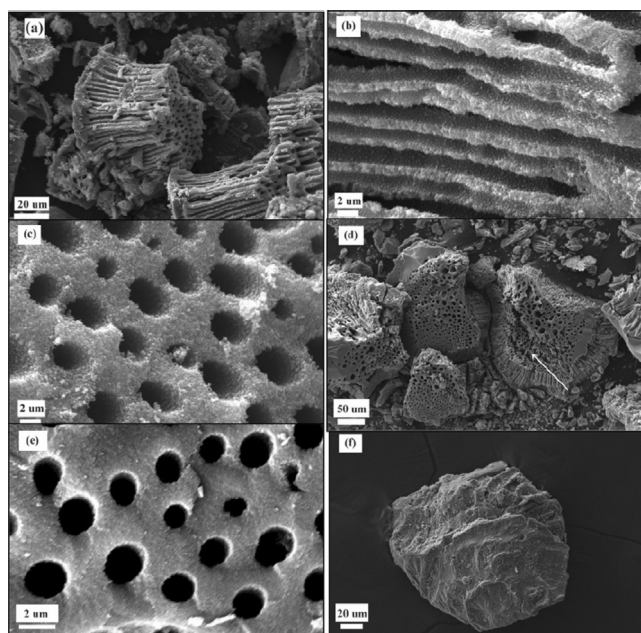
Figure 16. SEM images of the \text{TiO}_2 monolithic particles calcined at a–c) 350 °C, d,e) 500 °C, and f) 650 °C. [83d] Copyright 2005 American Chemical Society.
