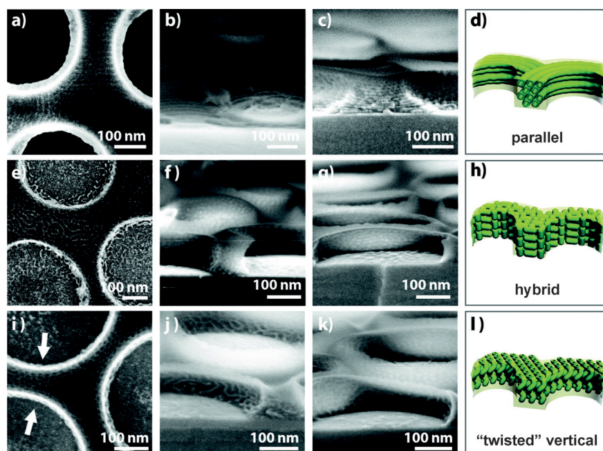
Figure 4. SEM images of textural mesoporosity of 3DOM \text{SiO}_2 : a–d) parallel mesopores formed with methanol as the solvent; e–h) transitional mesophases with methanol/water co-solvents; and i–l) possibly vertical mesophase and spherical mesopores formed in water. [25] Copyright 2012 American Chemical Society.
