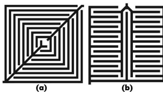
Figure 24. a) Leaf- and b) lung-inspired, biomimetic flow field designs. The inlet is at the top and the outlet is at the bottom. [133b] Reprinted from Ref. [133b] with permission from Elsevier.
