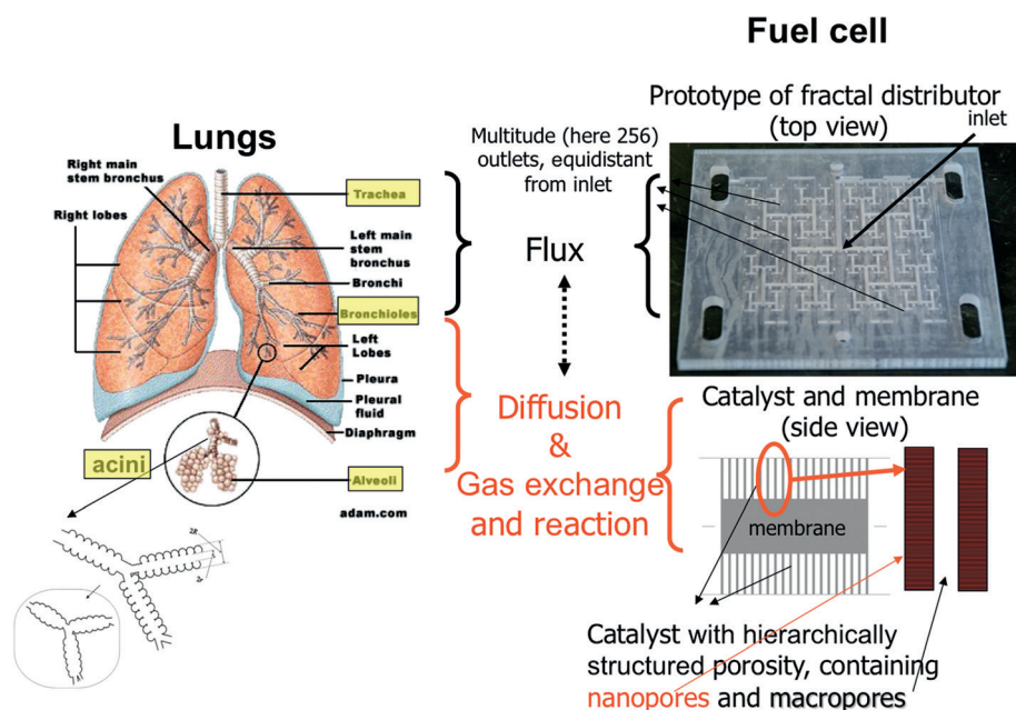
Figure 26. Fuel cell design guided by the architecture of the lung and the associated physical mechanisms. Based on Ref. [8c].
