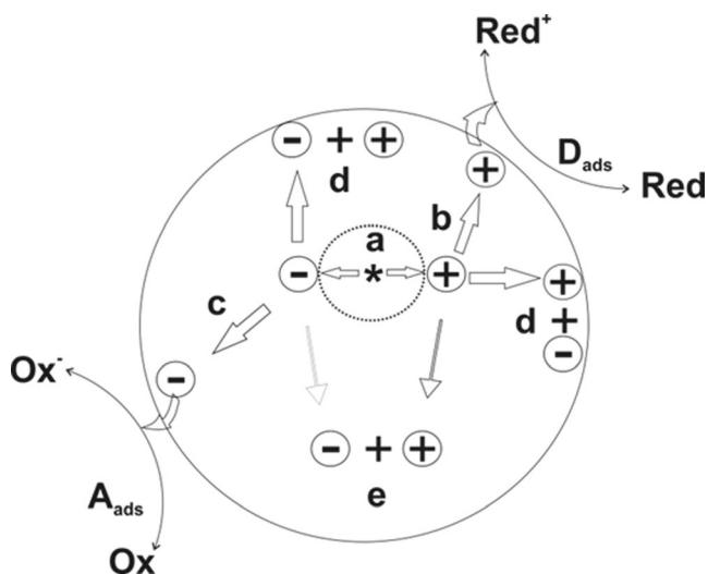
Figure 15. Main processes occurring on a semiconductor particle: a) electron-hole generation; b) oxidation of donor (D); c) reduction of acceptor (A); d,e) electron-hole recombination at surface and in bulk, respectively.
