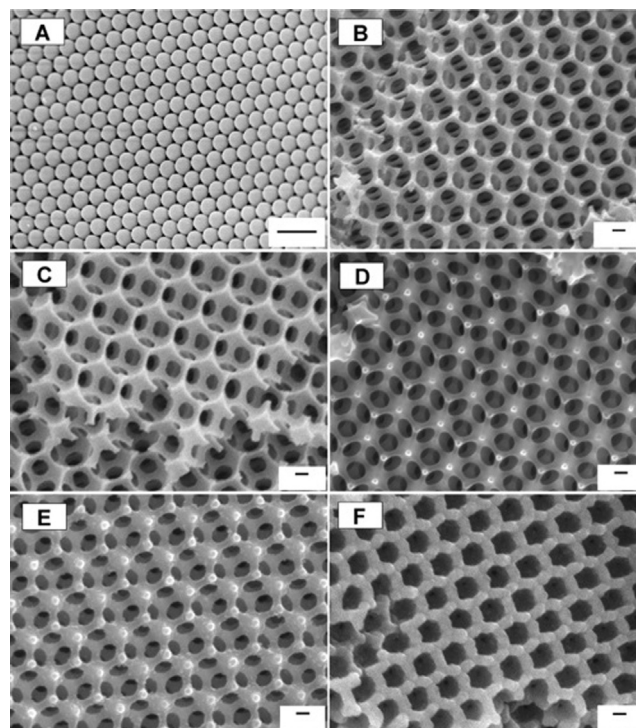
Figure 12. SEM images at different processing stages of 3DOM carbon: A) PMMA colloidal crystal template (scale bar: 1 \mu m); B) 3DOM/m SiO 2 monolith synthesized with PMMA as template (scale bar: 100 nm); C) 3DOM/m Al-SiO 2 monolith, obtained from aluminum impregnation of the 3DOM/m SiO 2 monolith (scale bar: 100 nm); D) 3DOM/mC, after introduction of polymer, carbonization, and removal of silica with HF (scale bar: 100 nm); E) Carbon/carbon nanocomposites-2 h; and F) Carbon/carbon nanocomposites-5 h carbon/graphite composite monoliths after CVD reaction times of 2 and 5 h, respectively (scale bar: 100 nm). [26a] Copyright 2006 American Chemical Society.
