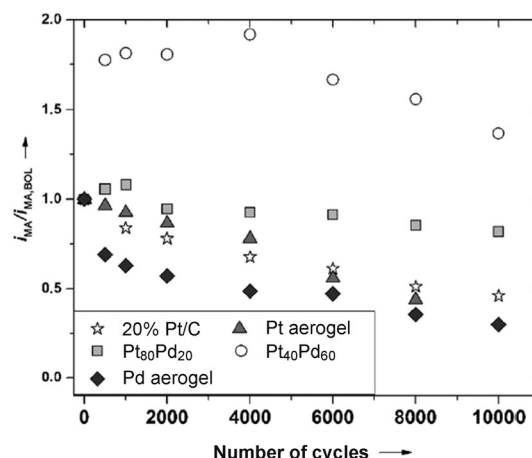
Figure 23. Relative ORR mass activity of Pt,Pd catalysts of different compositions as a function of the number of potential cycles (0.5 V to 1.0 V). The mass activity was obtained from the cathodic scan of ORR polarization curves (corrected for electrolyte resistances) at 10 \text{ mV s}^{-1} and 1600 rpm. [45c] Copyright 2013 Wiley.
