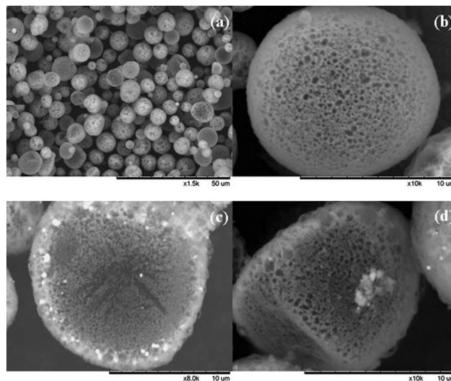
Figure 14. SEM images of a) 3D nanoporous \text{LiFePO}_4/\text{C} spheres; b) the surface of a single sphere; and c,d) cross-sections of spheres, showing the interconnected pores. [63] Scale bars: a) 50 \mu\text{m} , b–d) 10 \mu\text{m} . Copyright 2011 Royal Society of Chemistry.
