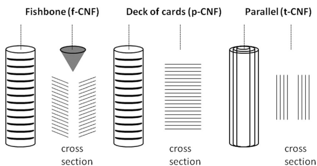
Figure 20. Schematic representation of three types of CNFs. Based on Ref. [122b].
